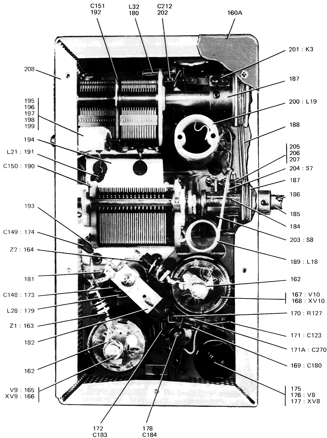
DETAIL C
