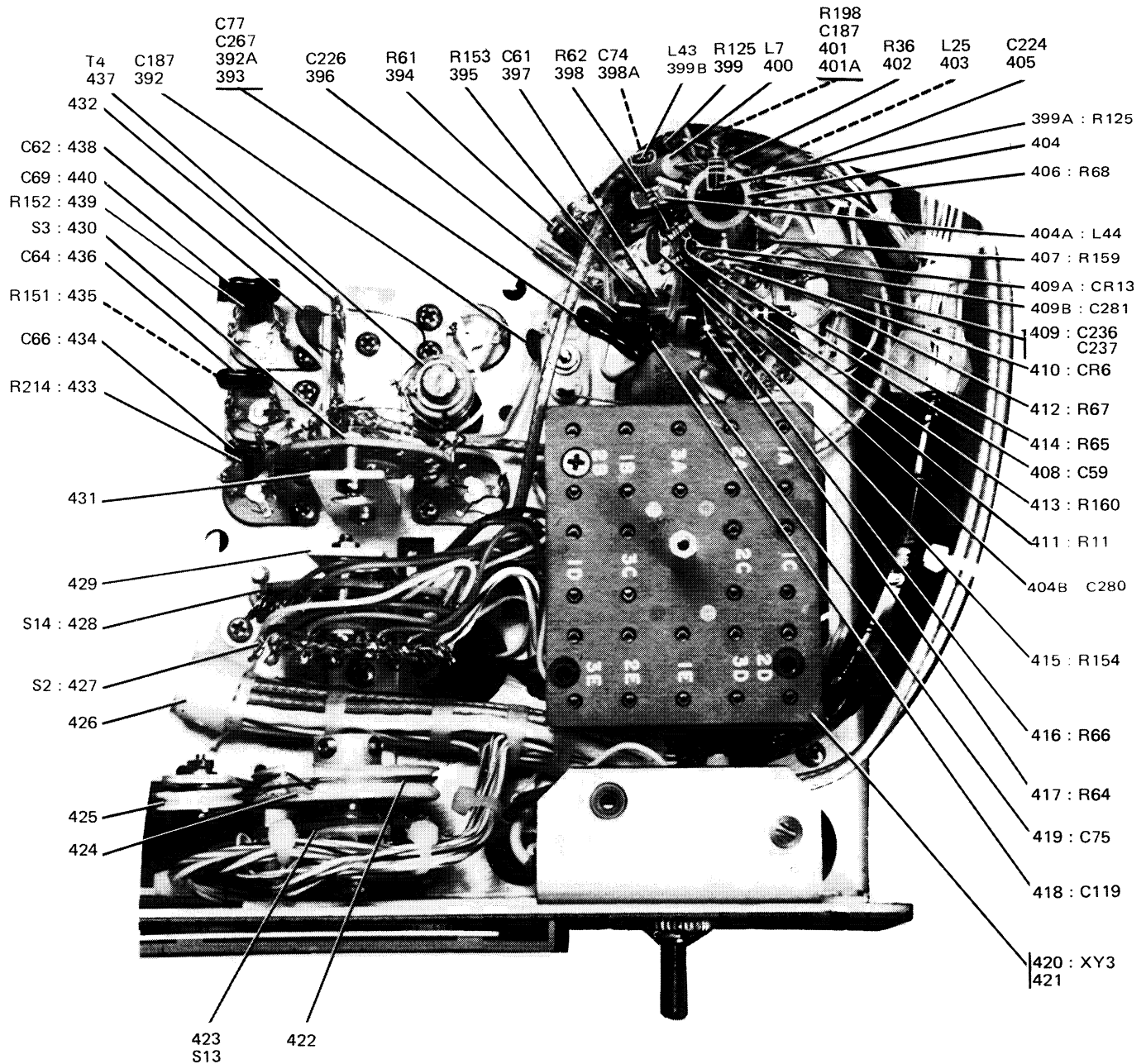
DETAIL H
