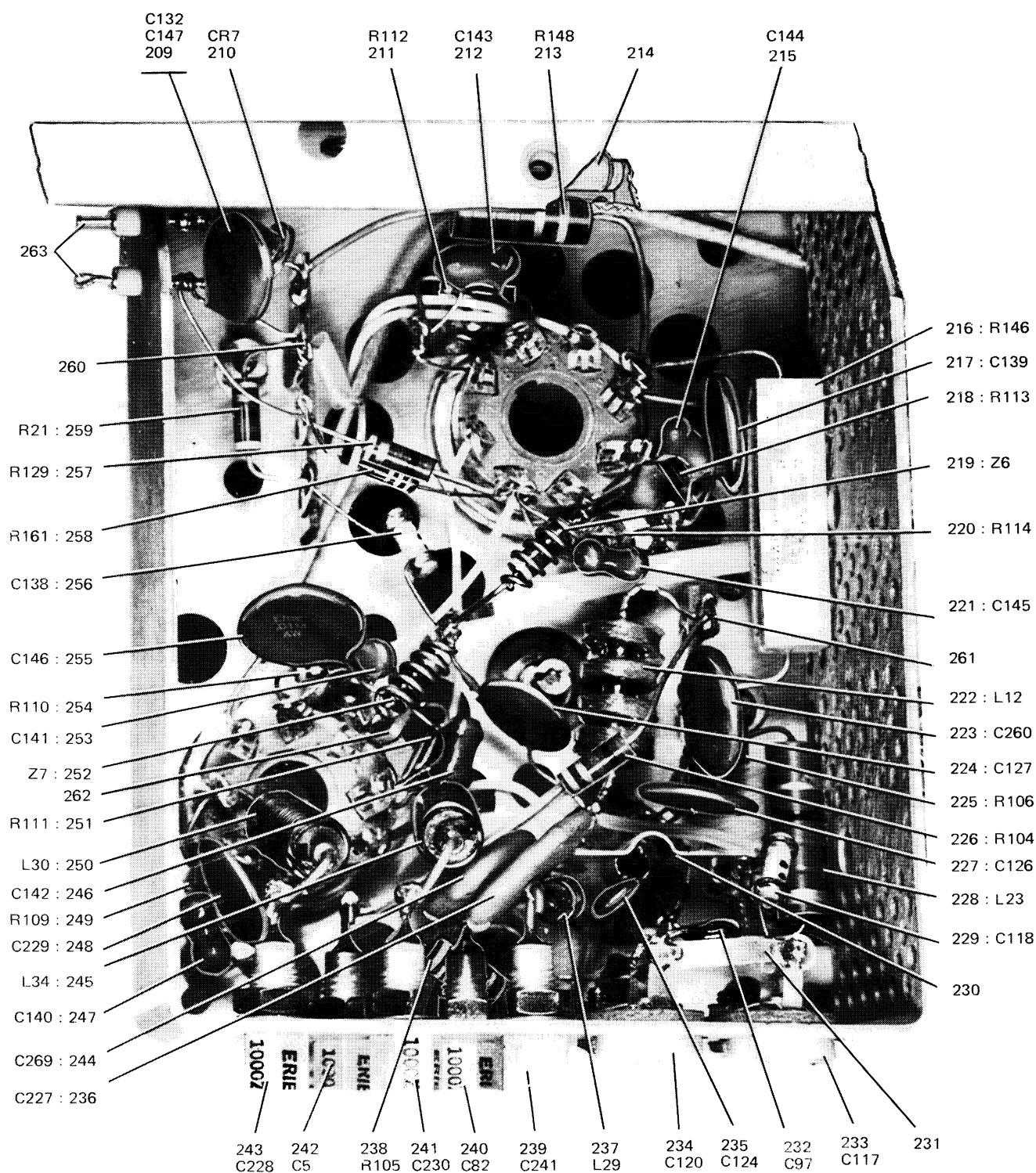
DETAIL D
