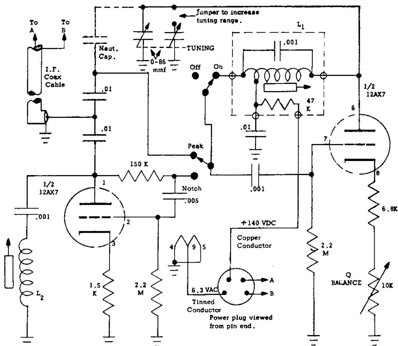
SCHEMATIC DIAGRAM OF 2-BQ
