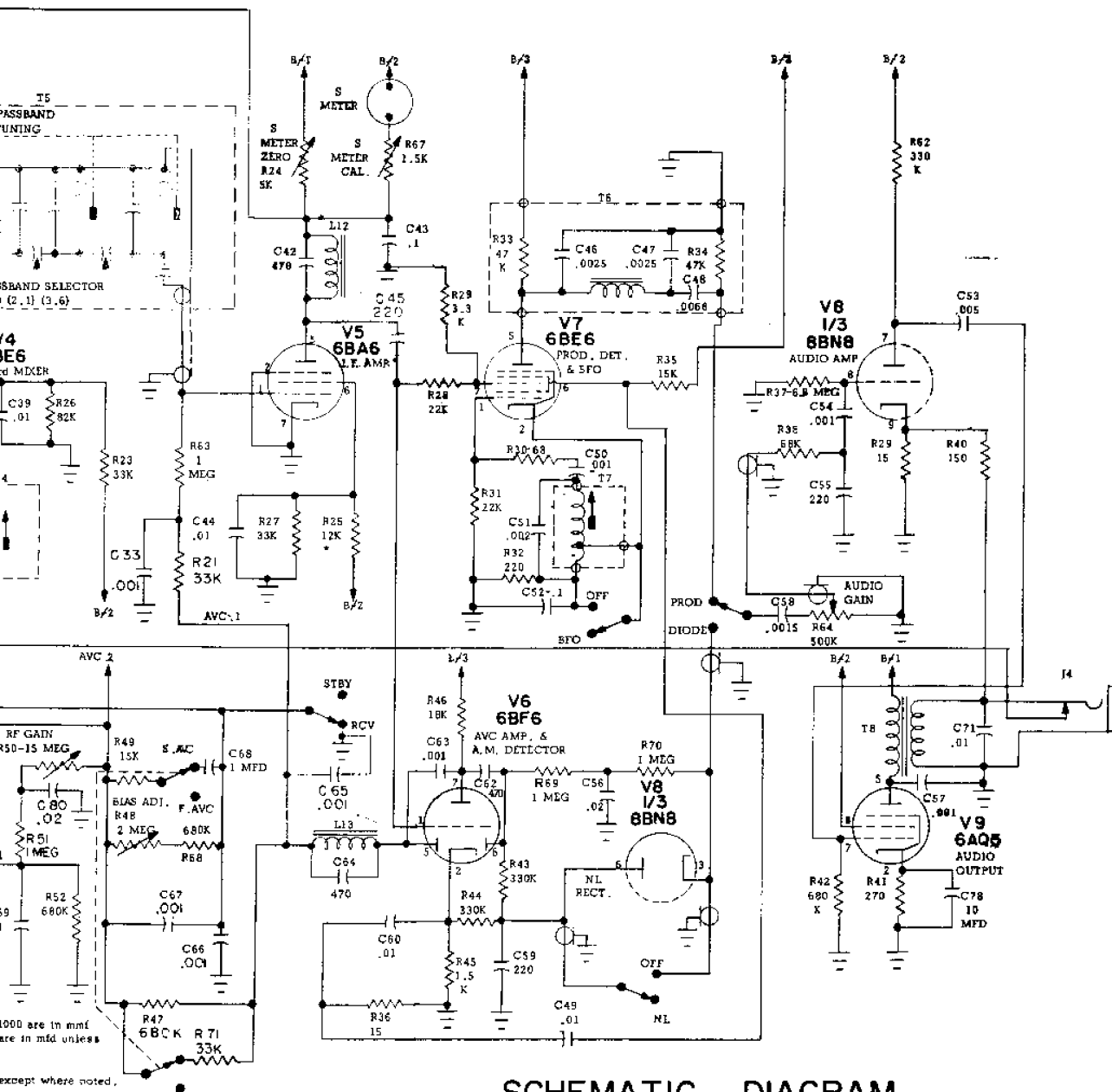
SCHEMATIC DIAGRAM MODEL 2-B COMMUNICATIONS RECEIVER
